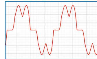
Non-Linear Load
